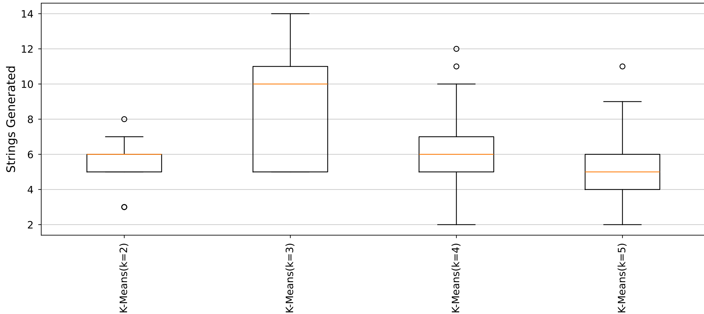
YARA Rules Strings Generated Distribution (Cluster38_Size5 dataset)
